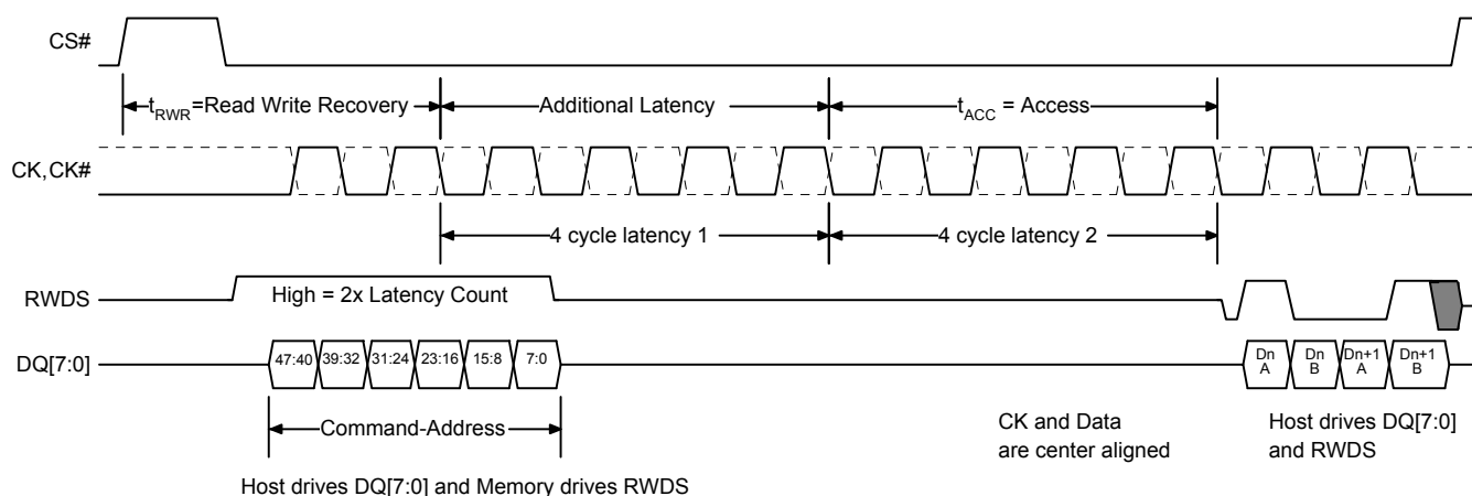
Figure 3.5 Write Transaction, Fixed Latency Mode
