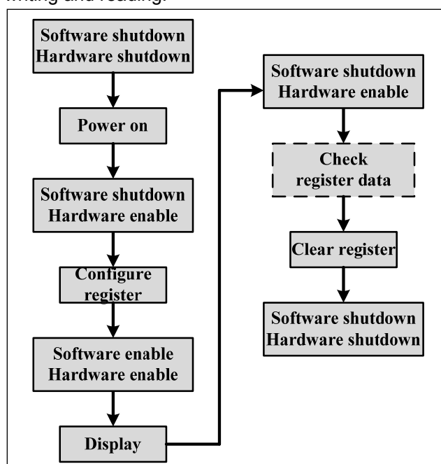
Figure 15 Shutdown Control
