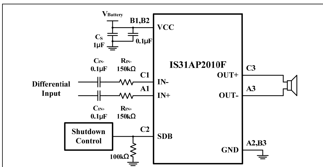
Figure 1 Typical Application Circuit (Differential Input)
