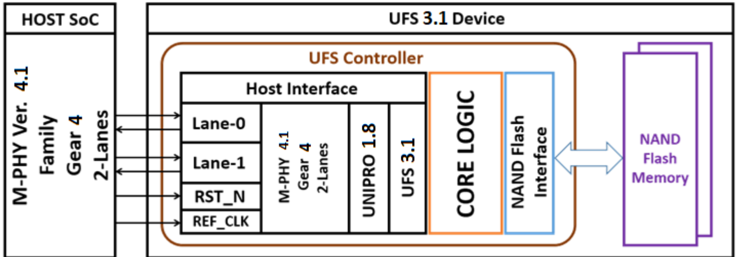
Figure 1-1 Device Block Diagram
