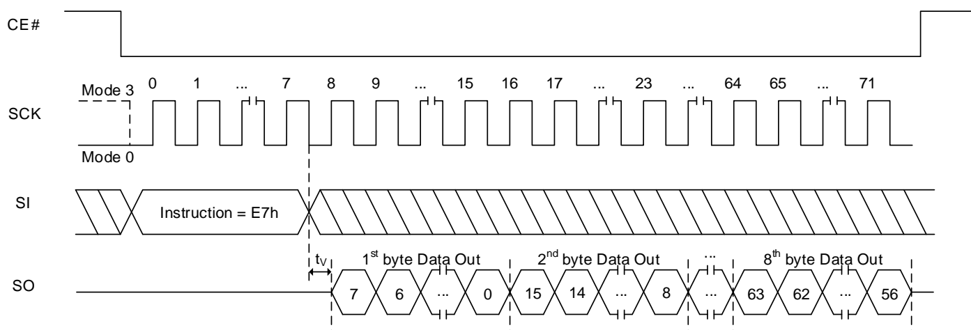
Figure 8.138 Read password Sequence In SPI Mode
