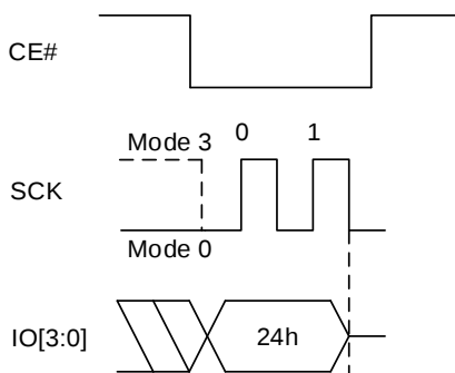
Figure 8.104 Sector Lock Sequence In QPI mode
