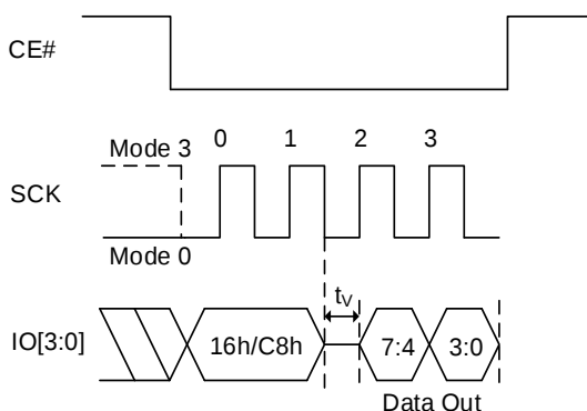
Figure 8.102 Read Bank Address Register Sequence In QPI Mode
