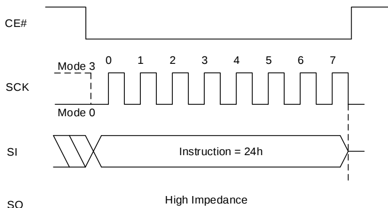
Figure 8.103 Sector Lock Sequence In SPI mode
