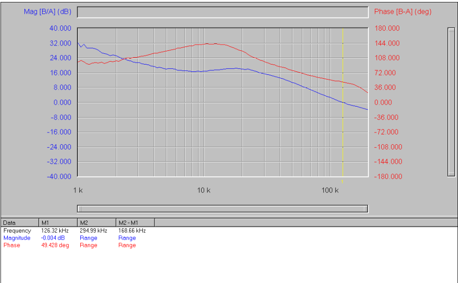
Bode plot-Sinking mode Vin-1.5V Vout-0.75V/4.3A
