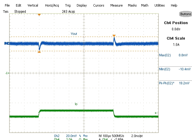
Transient response-Sinking mode Vin-1.35V Vout-0.675V/2.5-2.9-2.5A Ch4-Vout Ch3-Iout (1A/μSec slew rate)
