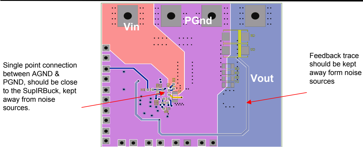
IRDC3898 demo board layout considerations – Bottom Layer
