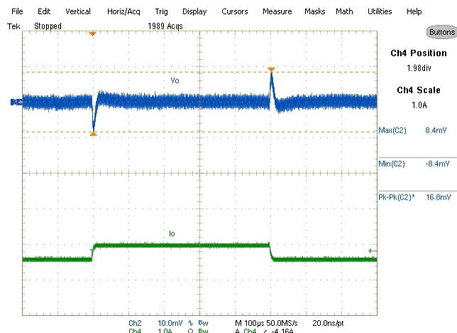
Transient response-Sinking mode Vin-1.35V Vout-0.675V/3.9-4.3-3.9A Ch4-Vout Ch3-Iout (1A/μSec slew rate)
