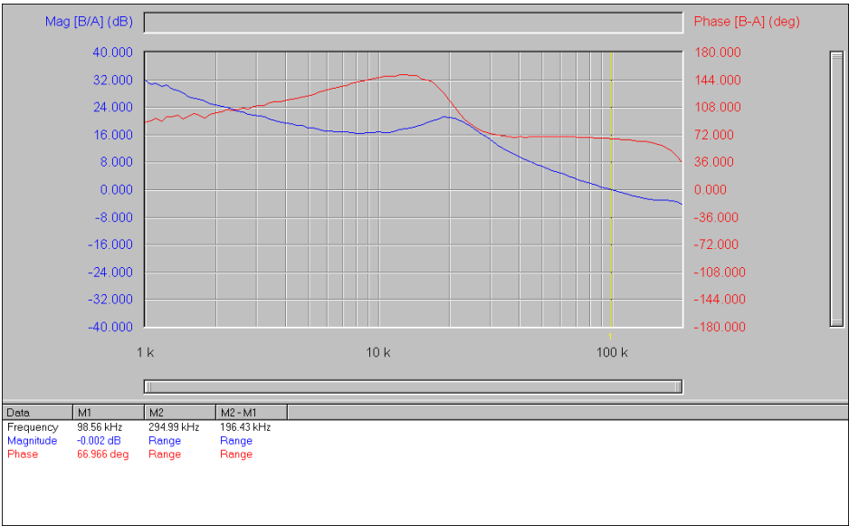
Bode plot-Sourcing mode Vin-1.5V Vout-0.75V/4.3A
