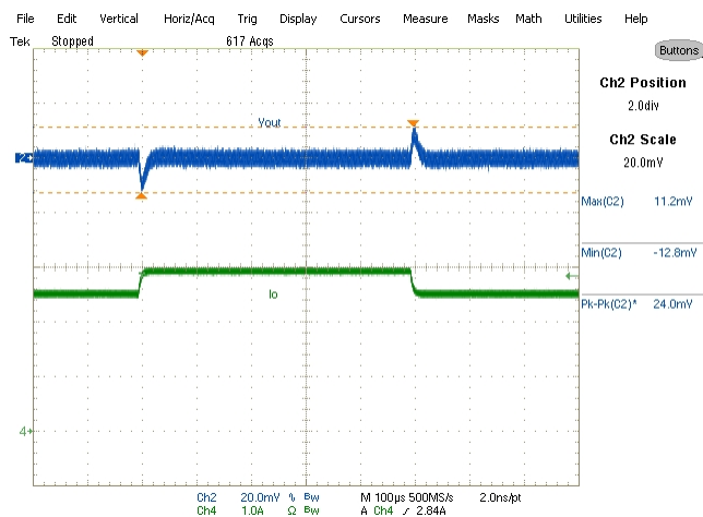
Transient response-Sourcing mode Vin-1.35V Vout-0.675V/2.5-2.9-2.5A Ch4-Vout Ch3-Iout (1A/μSec slew rate)
