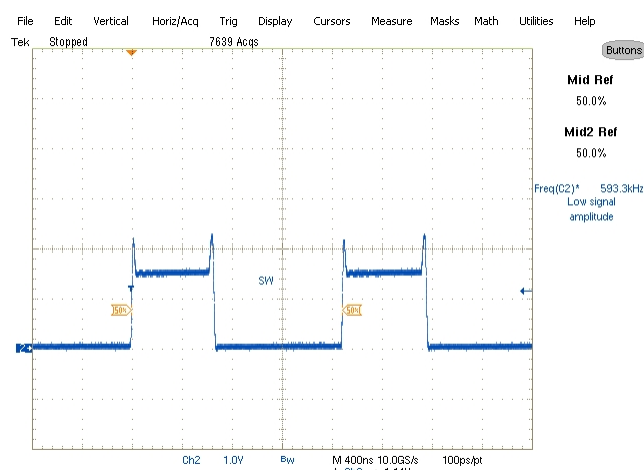
Switch node Voltage (20MHz BW)-Sinking mode Vin-1.5V Vout-0.75V/4.3A
