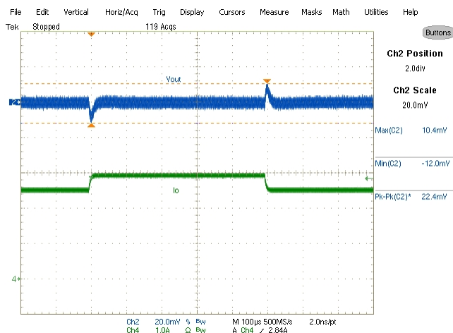
Transient response-Sourcing mode Vin-1.5V Vout-0.75V/2.5-2.9-2.5A Ch4-Vout Ch3-Iout (1A/μSec slew rate)
