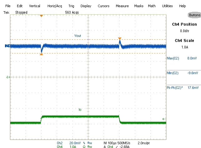
Transient response-Sinking mode Vin-1.5V Vout-0.75V/2.5-2.9-2.5A Ch4-Vout Ch3-Iout (1A/μSec slew rate)
