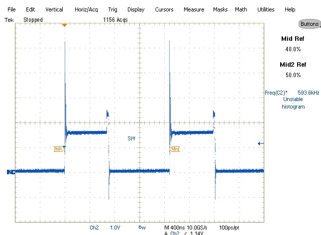
Switch node Voltage (250MHz BW)-Sinking mode Vin-1.5V Vout-0.75V/4.3A
