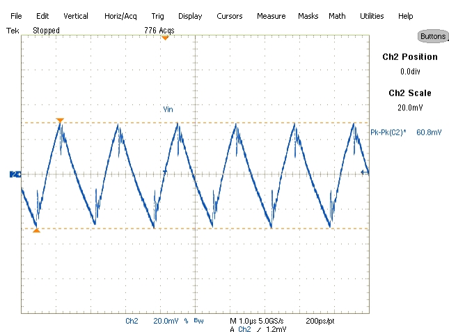
I/P Ripple Voltage-Sinking mode Vin-1.35V Vout-0.675V/4.3A
