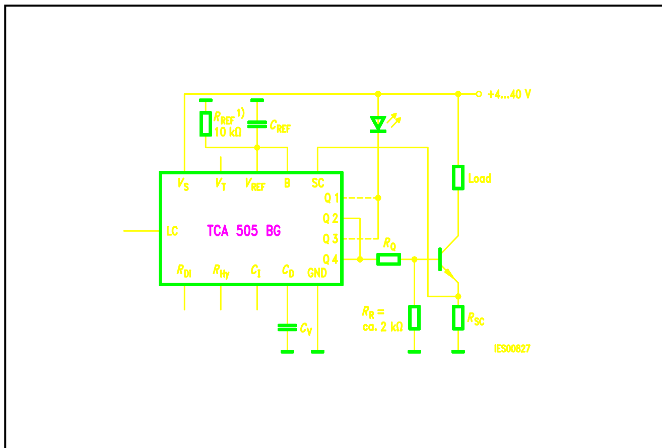
Application Circuit 3
