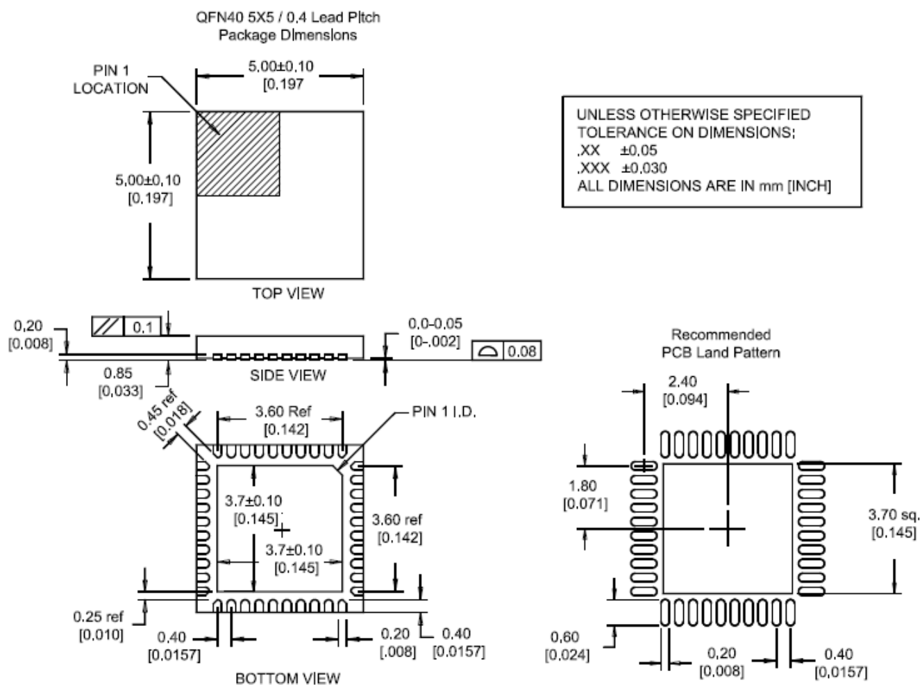
Figure 61: Package Dimensions
