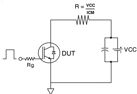
Fig.C.T.2 - RBSOA Circuit
