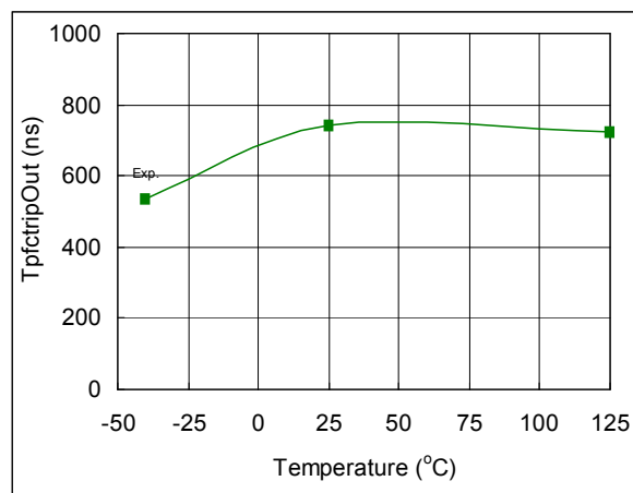
Fig. 75. PFC TRIP to Output Shutdown Propagation Delay
