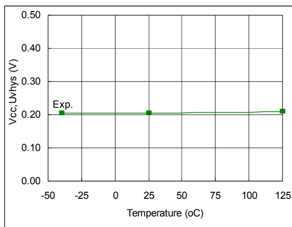
Fig. 108. V_{CC} Supply Undervoltage Hysteresis vs. Temperature
