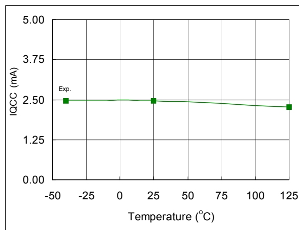
Fig. 50. Quiescent V CC Supply Current vs. Temperature
