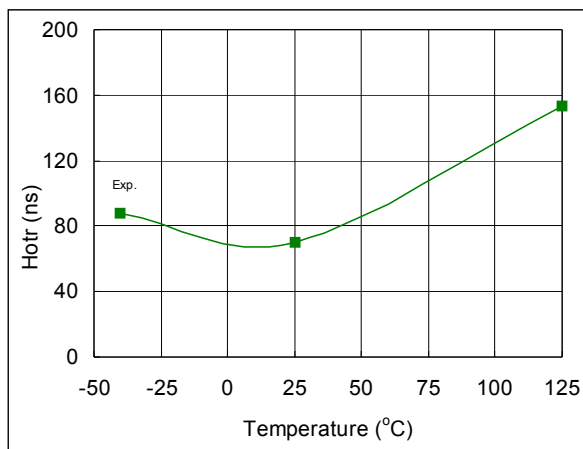
Fig. 58. Turn-On Rise Time vs. Temperature
