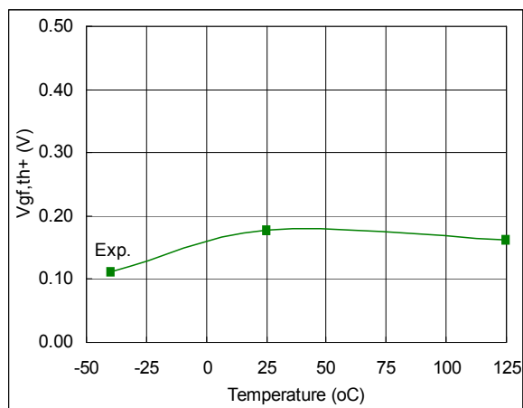
Fig. 104. GF Positive Going Threshold vs. Temperature
