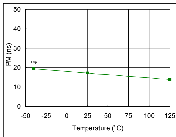
Fig. 67. Pulse Width Distortion vs. Temperature
