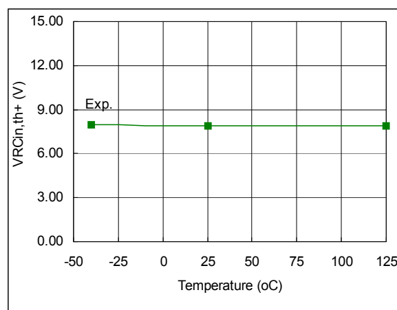
Fig. 105. RCIN Positive Going Threshold vs. Temperature
