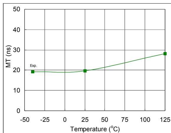
Fig. 65. Ton, Off Matching Time vs. Temperature
