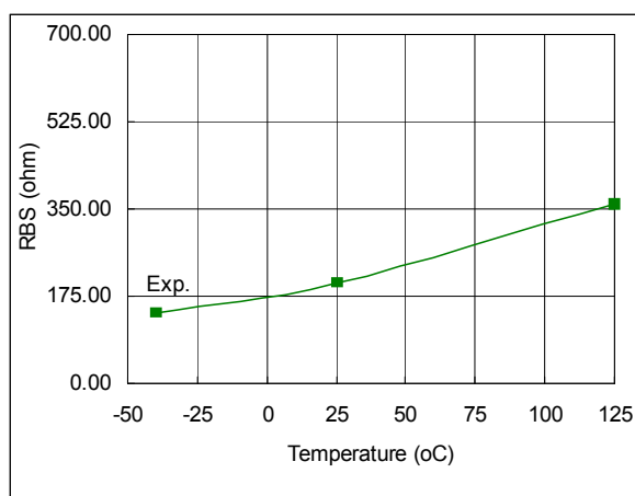
Fig. 116. Ron Internal Bootstrap Diode vs. Temperature
