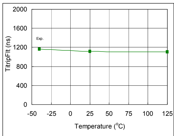
Fig. 69. ITRIP to Fault Time vs. Temperature
