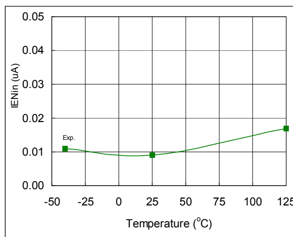
Fig. 117. En Input Bias Current vs. Temperature
