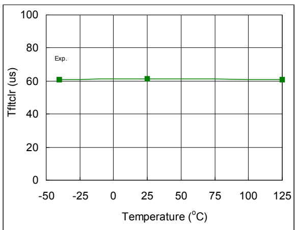
Fig. 72. FAULT Clear Time RCIN vs. Temperature
