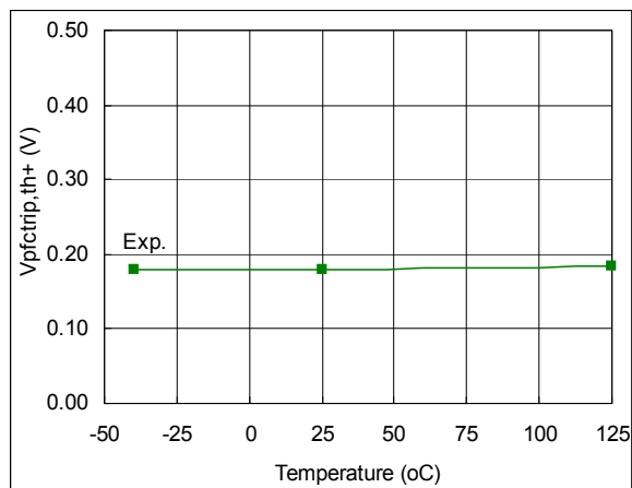
Fig. 102. PFC Positive Going Threshold vs. Temperature
