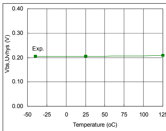
Fig. 109. V_{BS} Supply Undervoltage Hysteresis vs. Temperature
