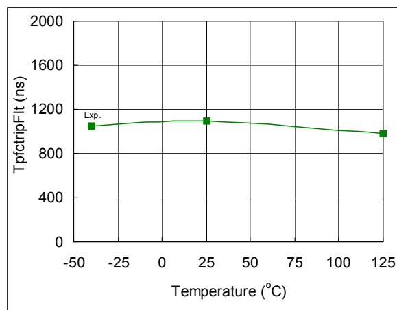
Fig. 74. PFC TRIP to Fault Time vs. Temperature
