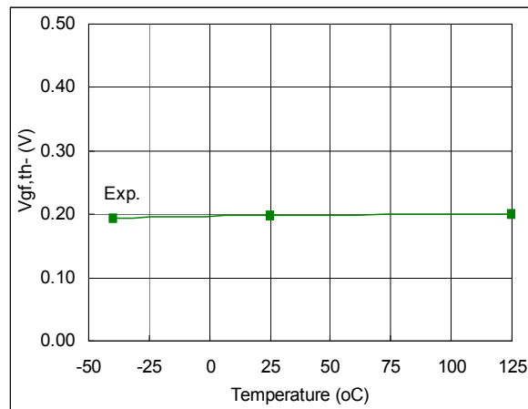
Fig. 103. GF Negative Going Threshold vs. Temperature
