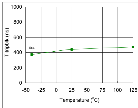
Fig. 73. ITRIP Blanking Time vs. Temperature
