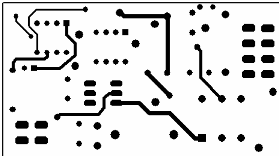
Top Copper
