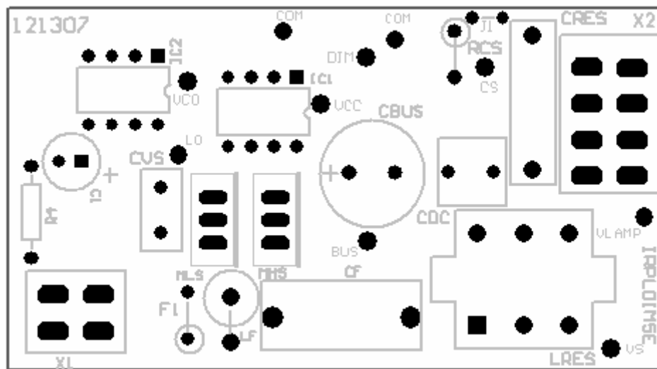
Top Assembly
