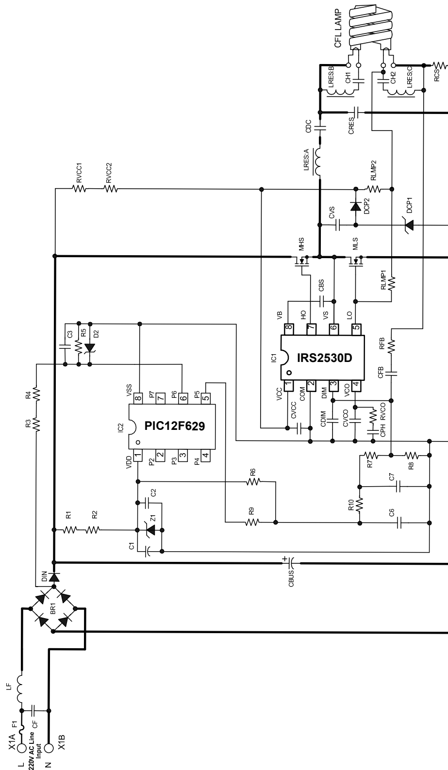
Figure 3.1: IRPLDIM5E Circuit Schematic
