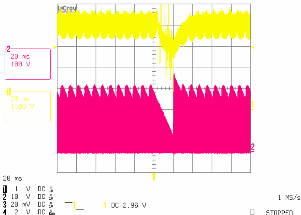
Figure 5.2: Brown-out conditions: CH1 is the VCO voltage, CH2 is the VS voltage
