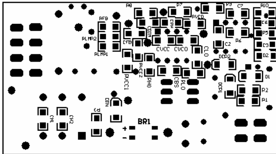
Bottom Assembly
