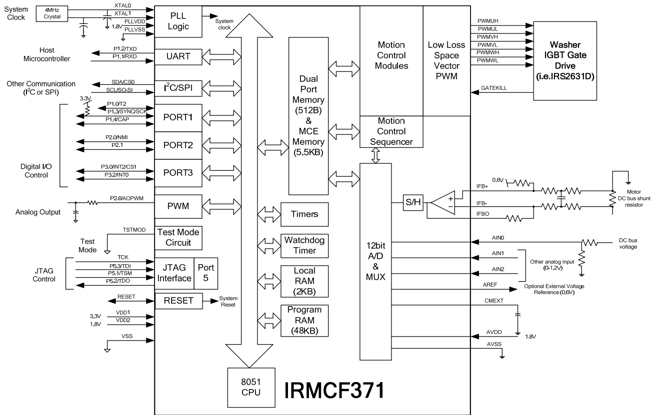
Figure 5. Application Connection of IRMCF371
