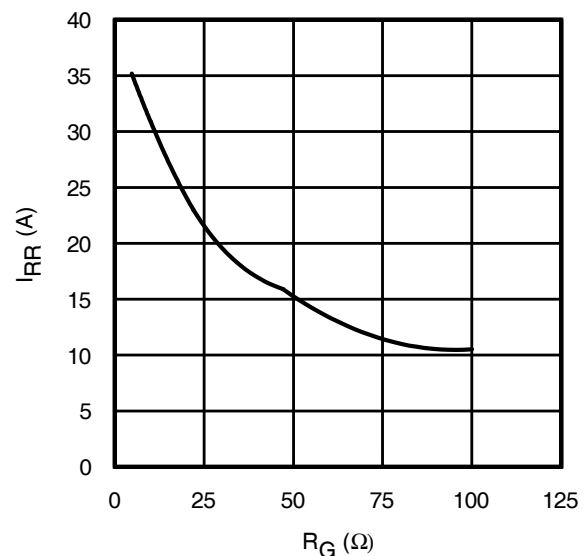
Fig. 19 - Typ. Diode I_{\text{RR}} vs. R_G
