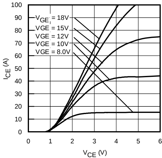
Fig. 5 - Typ. IGBT Output Characteristics T j = -40°C; tp = 300μs
