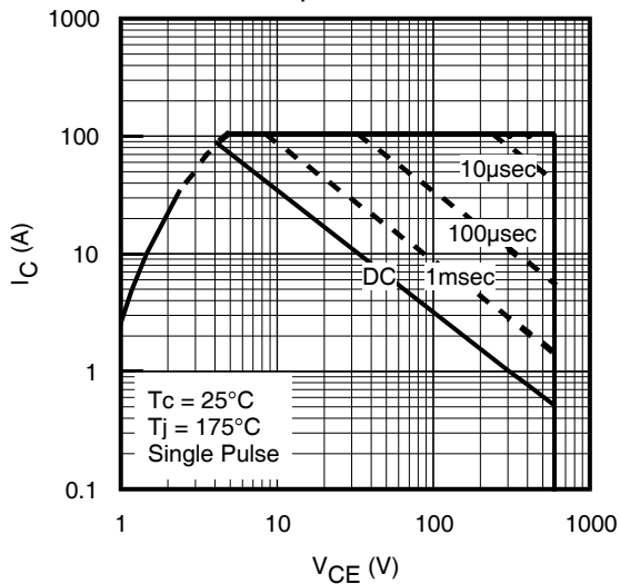
Fig. 4 - Forward SOA T C = 25°C; T J ≤ 175°C; V GE = 15V
