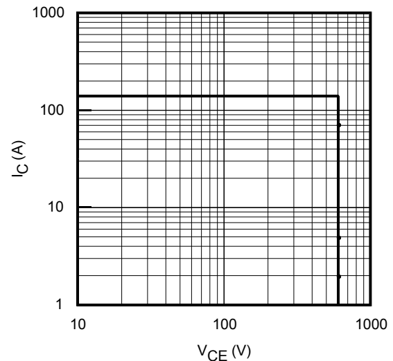
Fig. 5 - Reverse Bias SOA T J = 175°C; V GE = 20V
