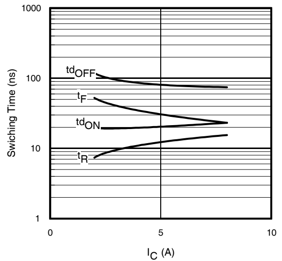
Fig. 14 - Typ. Switching Time vs. I_C T_J = 175^\circ\text{C} ; L = 1\text{mH} ; V_{CE} = 400\text{V} R_G = 100\Omega ; V_{GE} = 15\text{V}
