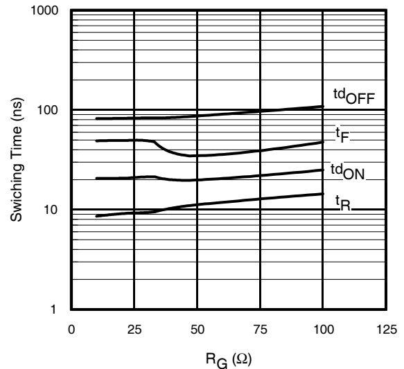
Fig. 16 - Typ. Switching Time vs. R_G T_J = 175^\circ\text{C} ; L = 1\text{mH} ; V_{CE} = 400\text{V} I_{CE} = 4\text{A} ; V_{GE} = 15\text{V}
