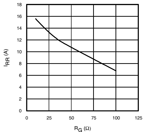
Fig. 18 - Typical Diode I_{RR} vs. R_G T_J = 175^\circ\text{C} ; I_F = 4.0\text{A}
