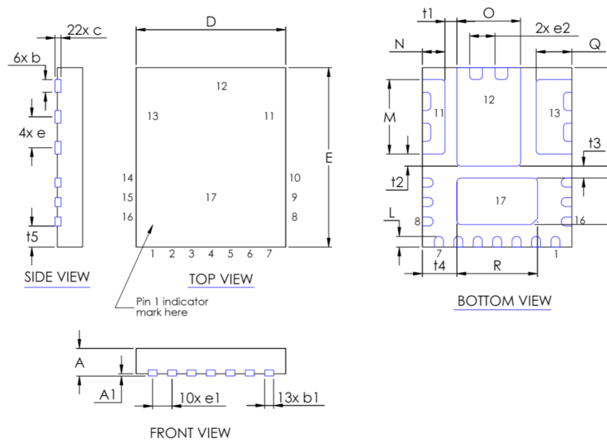
Figure 20: Package Dimensions
