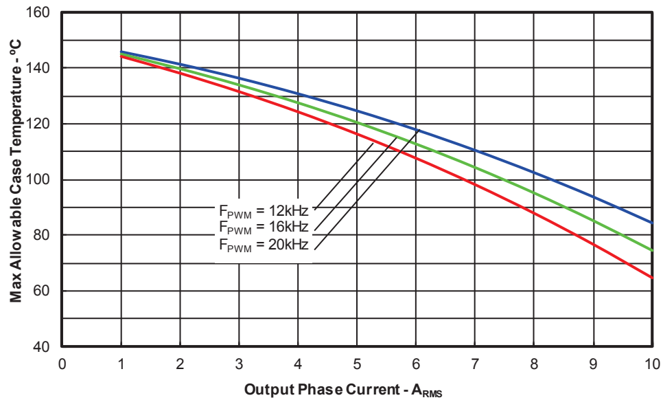
Figure 8. Maximum Allowable Case Temperature vs. Output RMS Current per Phase Sinusoidal Modulation, V + =400V, T J =150°C, MI=0.8, PF=0.6, f mod =50Hz
