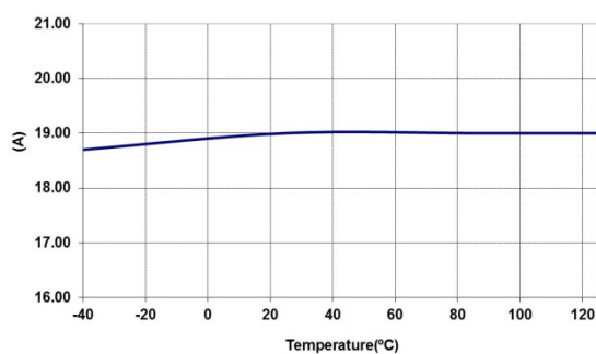
I_{OCP} with V_{in} = 5.0V , Internal LDO, f_{sw}=600\text{ kHz}
