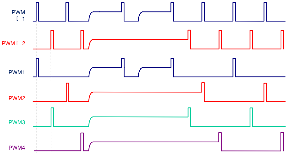
Figure 6: IR3599 timing when configured in DOUBLER mode (Industry Standard Tri-state PWM signals at input)
