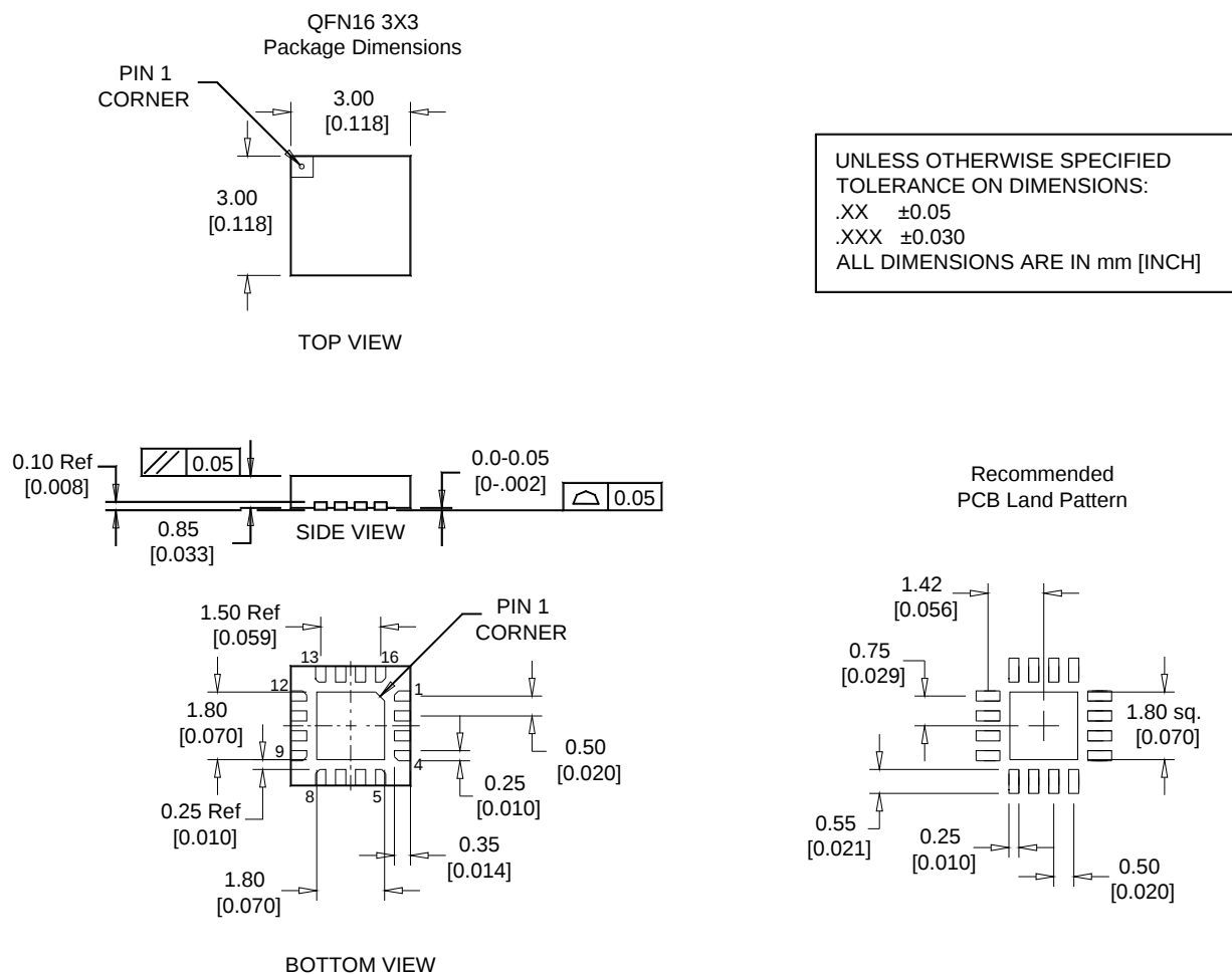
Figure 11: Package Dimensions
