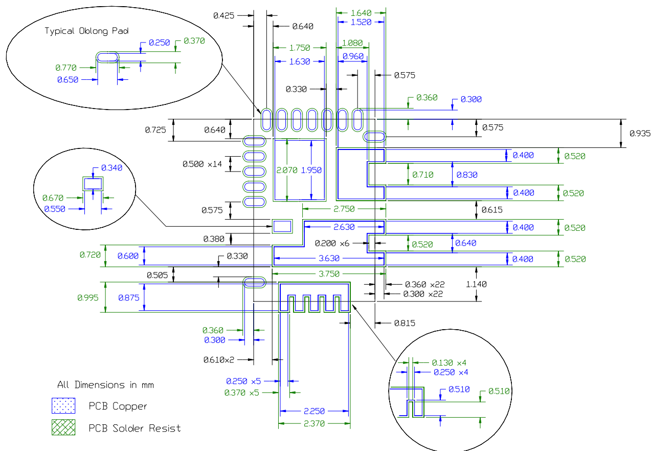
Figure 34: Solder resist
