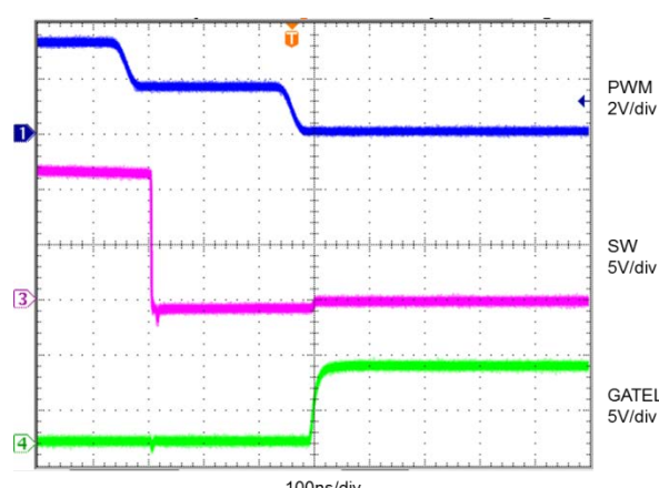
Figure 24: Tristate Delay in PWM Mode, 10A
