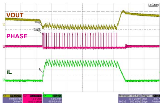
Figure 17: Load Transient 0-8A
