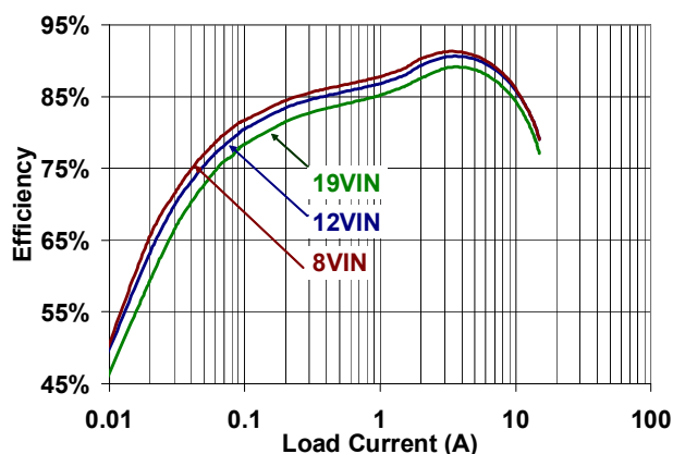
Figure 2: IR3477 Efficiency
