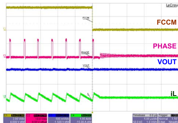
Figure 20: FCCM/DCM Transition
