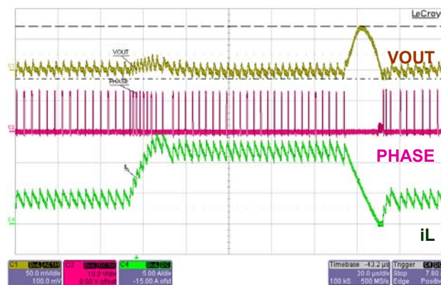
Figure 18: Load Transient 4-12A
