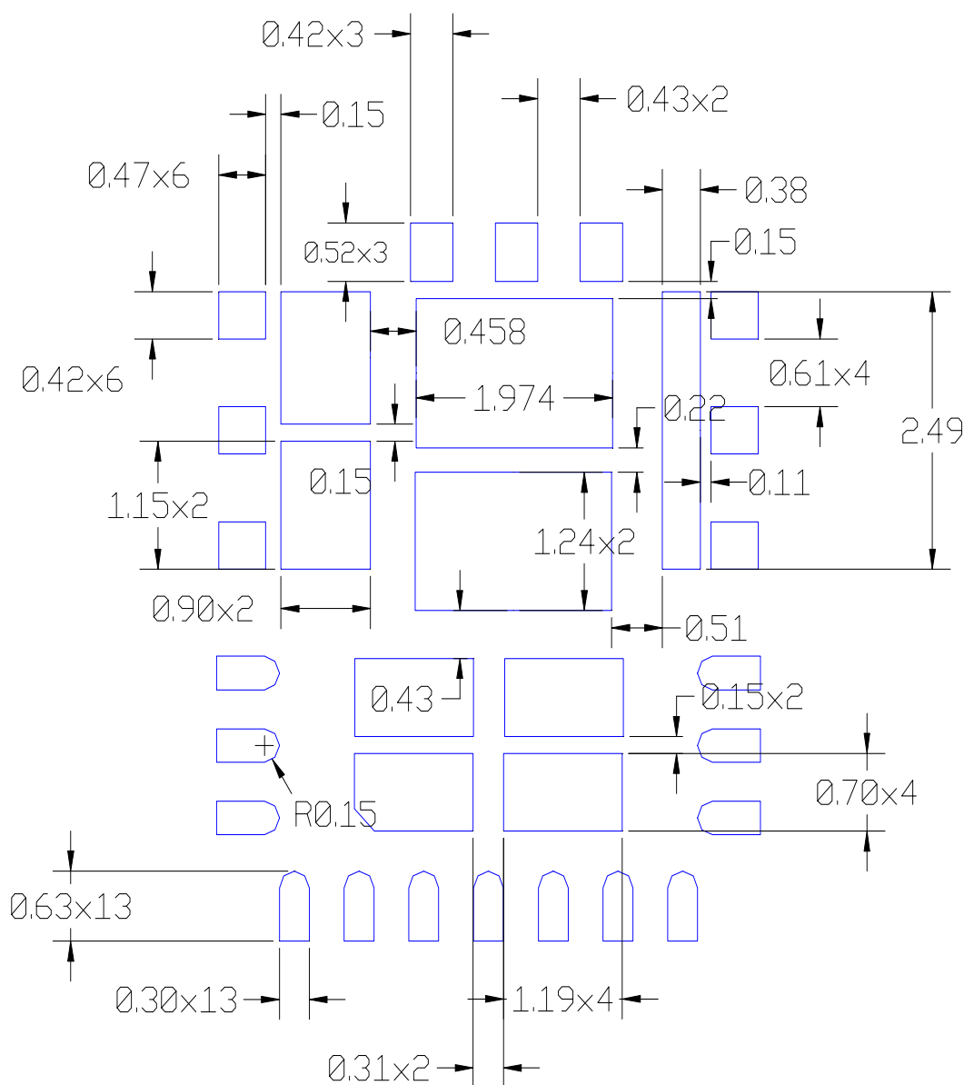
Figure 33: Stencil Design
