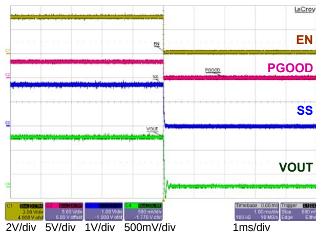
Figure 12: Shutdown
