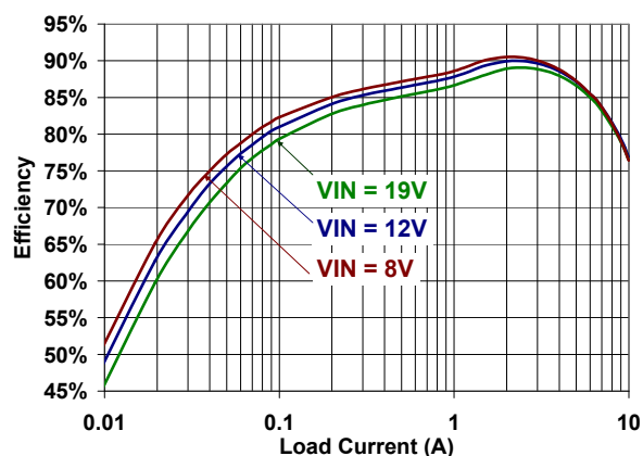
Figure 2: IR3475 Efficiency
