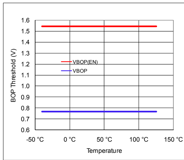
Figure 12: Brown-Out Protection Thresholds vs. Temperature
