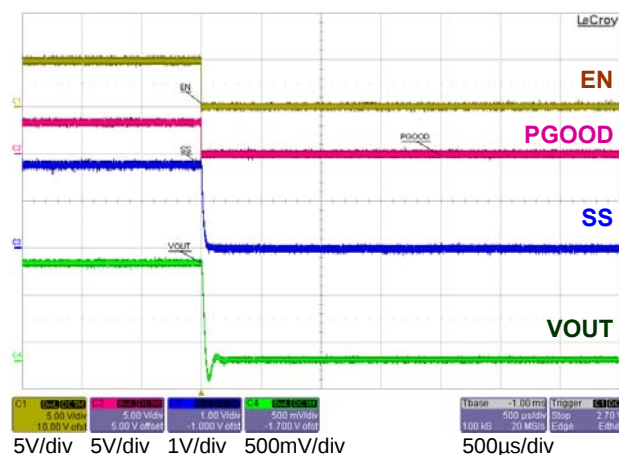
Figure 12: Shutdown
