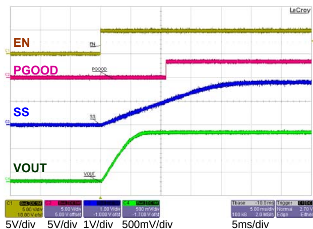
Figure 11: Startup
