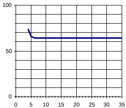
Figure 7 - R ds(on) (mΩ) Vs V cc (V)
