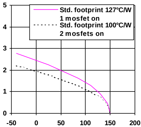
Figure 13 - Max.Cont. I_{ds} (A) Vs Amb. Temperature ( ^{\circ}\text{C} )
