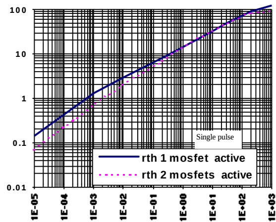
Figure 16 - Transient Thermal Imped. ( ^{\circ}\text{C/W} ) Vs Time (s)
