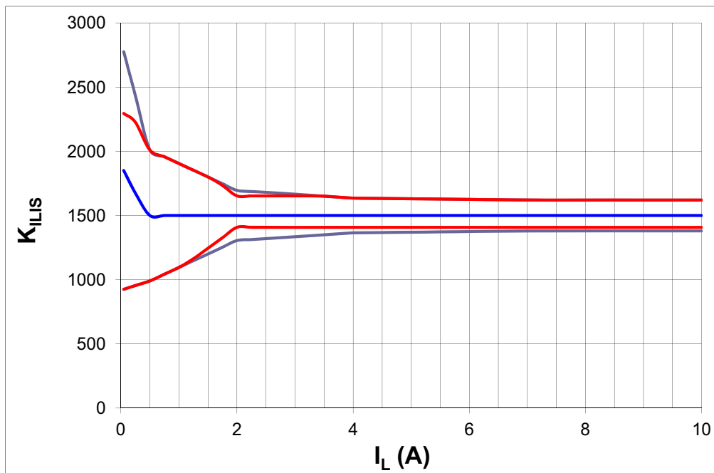
Figure 22 Improved Current Sense Accuracy with One Calibration Point
