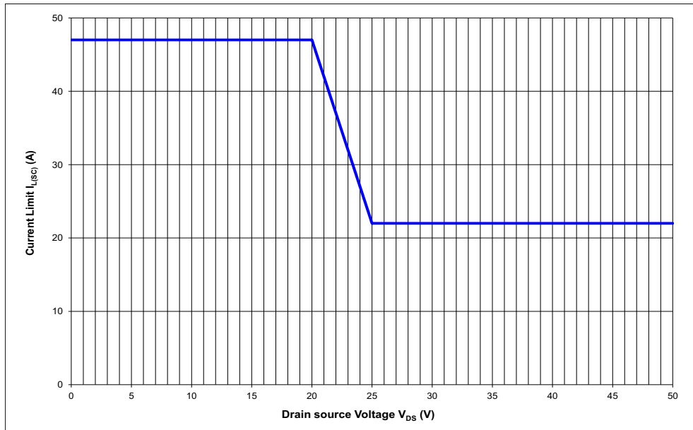
Figure 18 Current Limitation (typical behavior)
