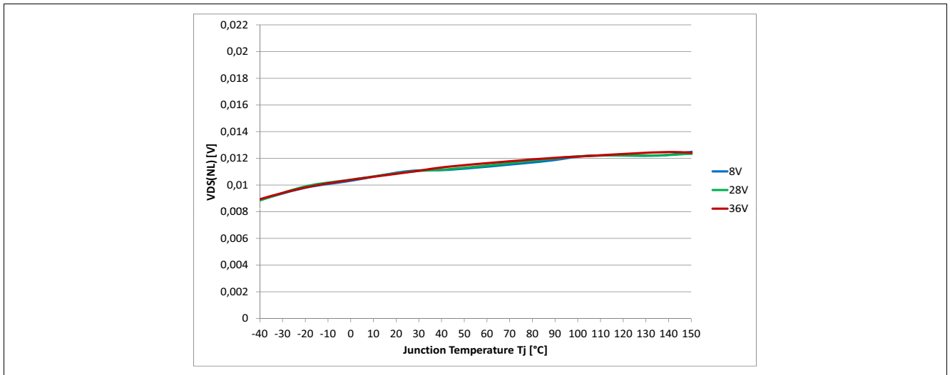
Figure 33 Output Voltage Drop Limitation at Low Load Current V_{DS(NL)} = f(T_J) and V_{DS(NL)} = f(V_{GS})
