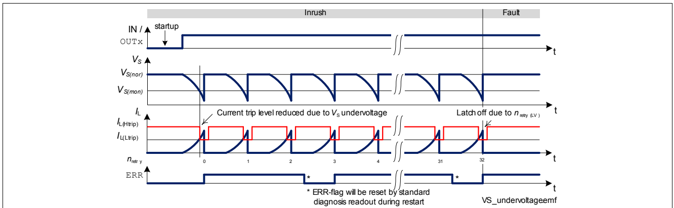
Figure 19 Behavior of current trip level in VS undervoltage condition
