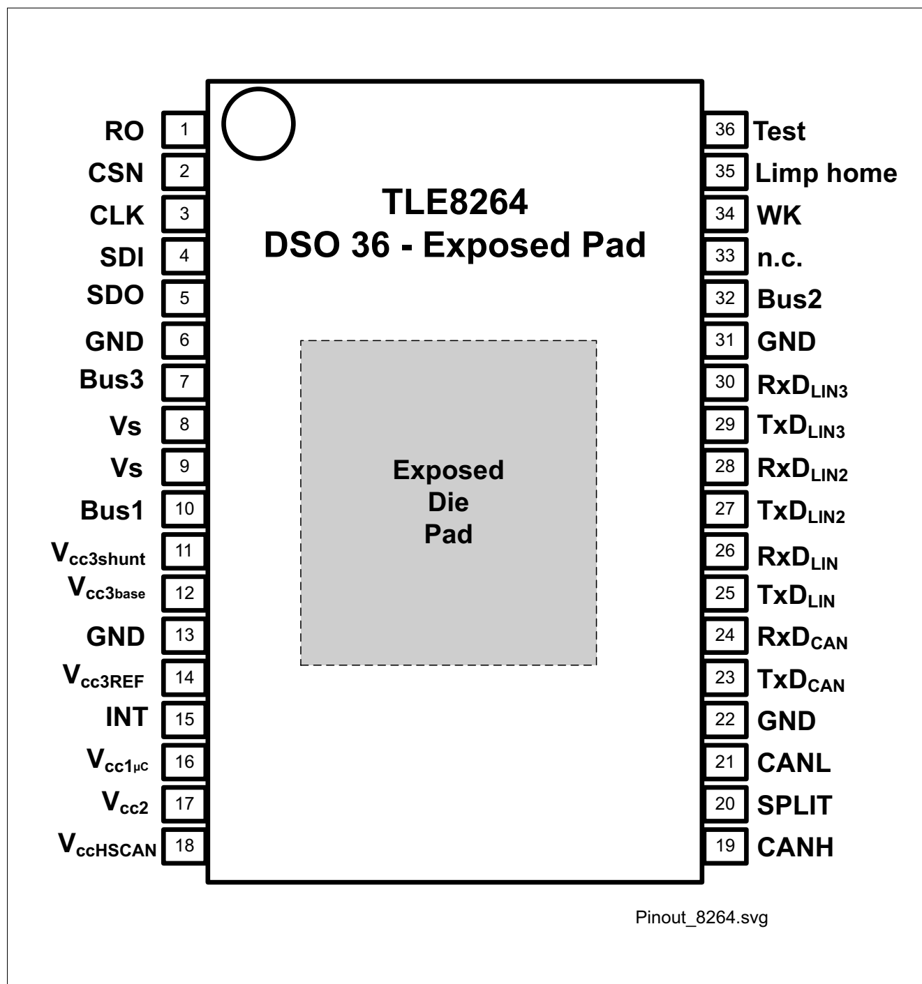
Figure 3 Pin Configuration
