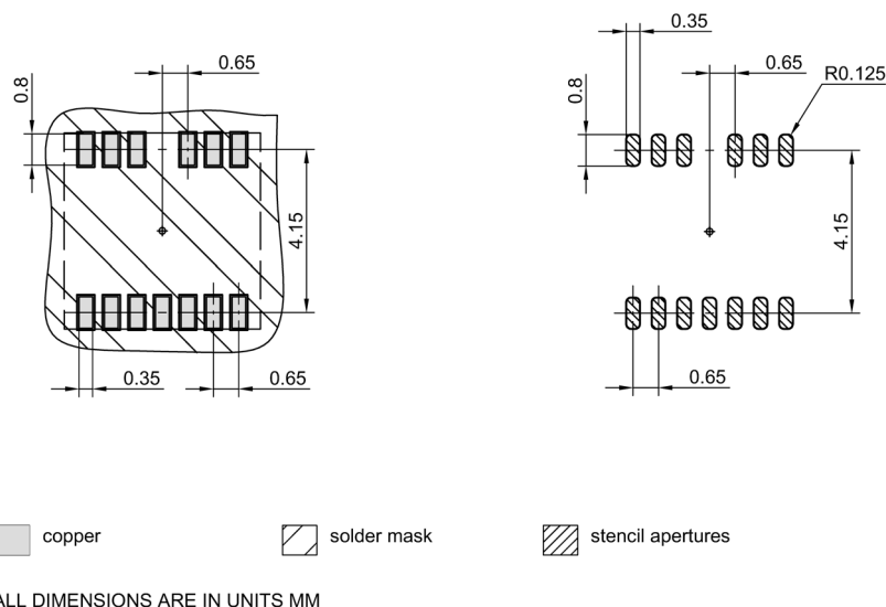
Figure 24 PG-TFLGA-13-1 footprint
