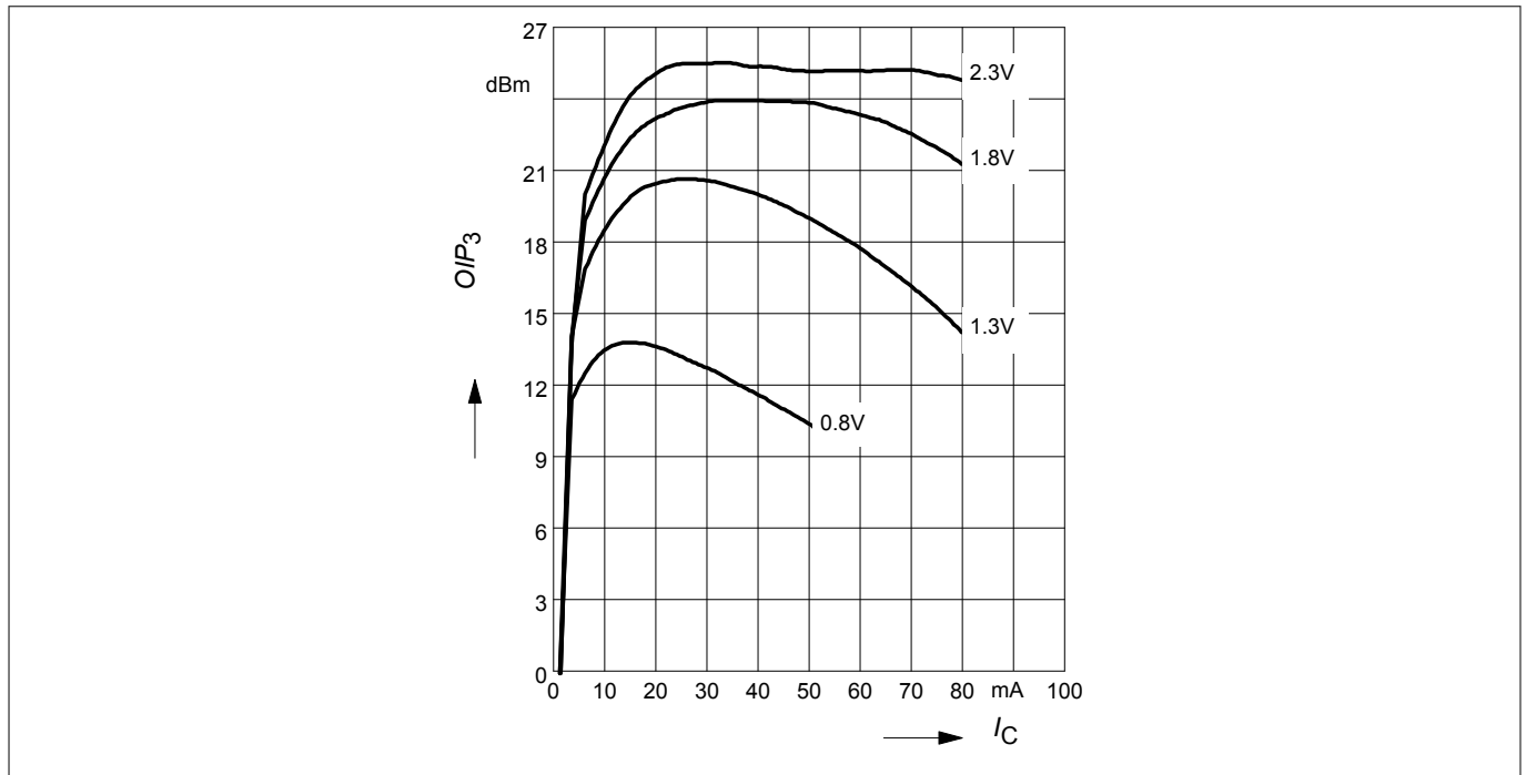
Figure 7 3rd order intercept point at output OIP_3 = f(I_C, V_{CE}) , Z_S = Z_L = 50 \Omega , f = 900 \text{ MHz}
