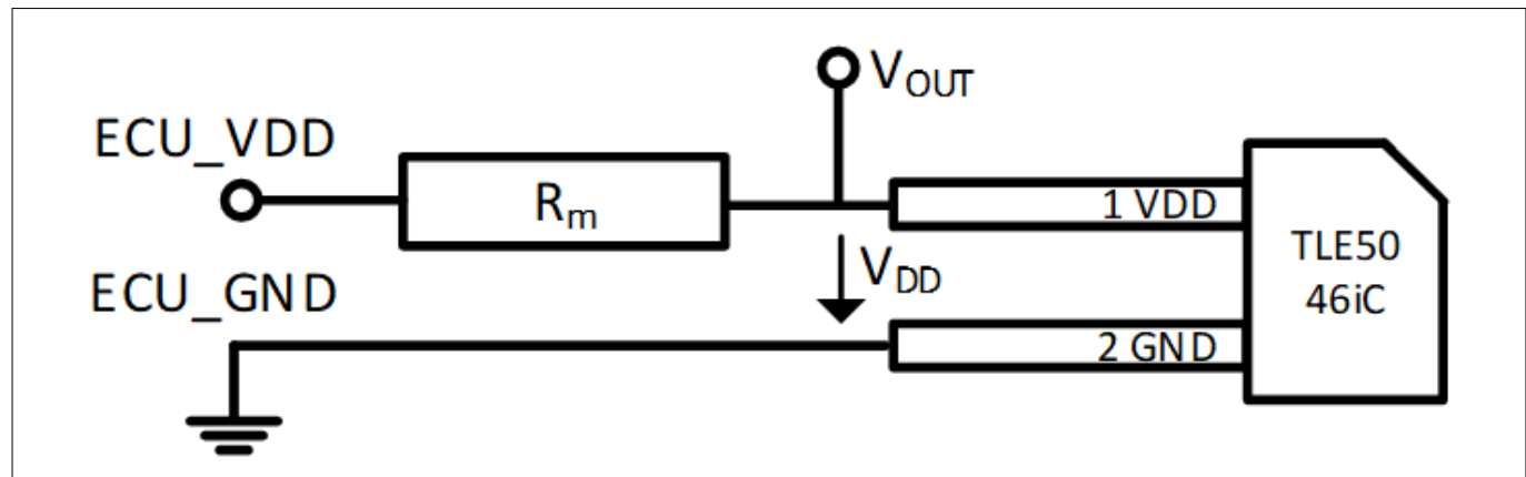
Figure 5 Pin configuration
