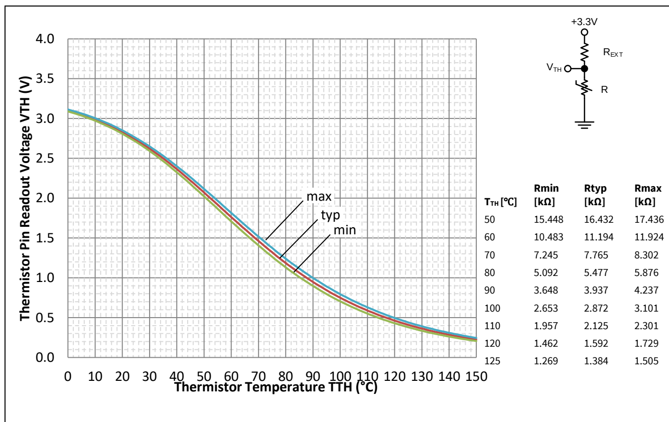
Figure 7 Thermistor resistance - temperature curve, for R_{EXT}=9.76k\Omega , and thermistor resistance variation with temperature.
