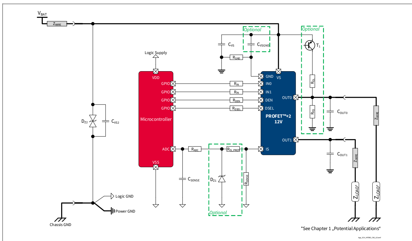
Figure 1 BTS7080-2EPZ Application Diagram. Further information in Chapter 10
