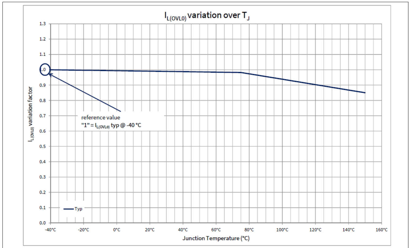
Figure 24 Overload Current Thresholds variation with T_J
