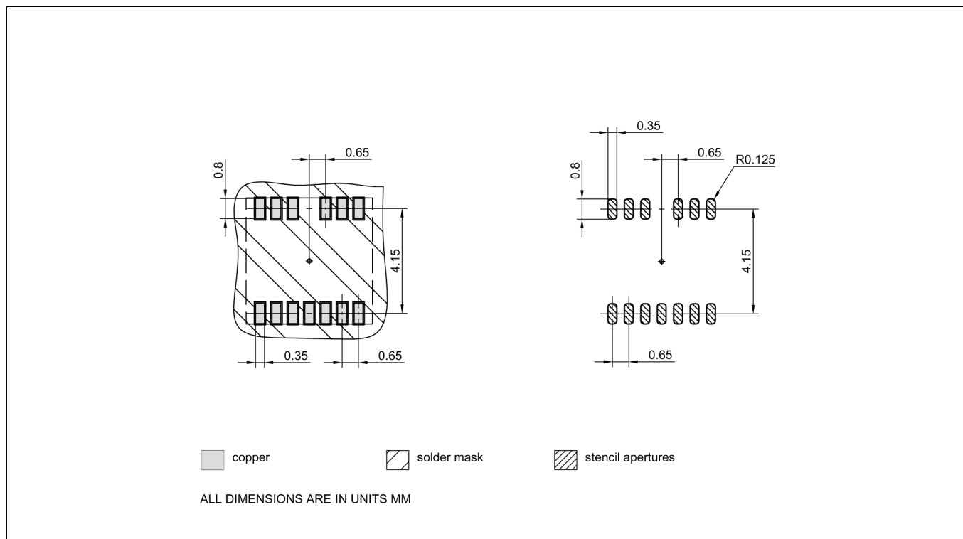
Figure 23 PG-TFLGA-13-1 footprint
