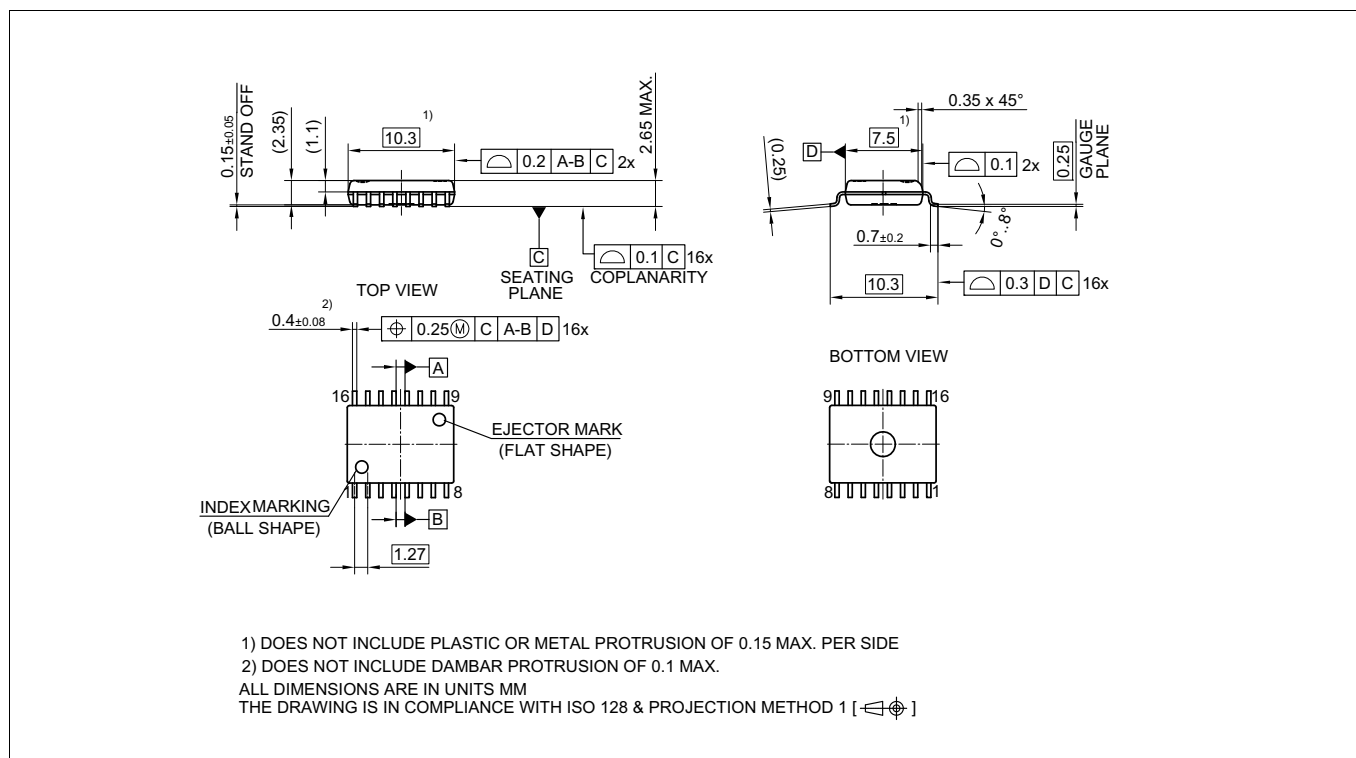
Figure 19 PG-DSO-16-30 outline
