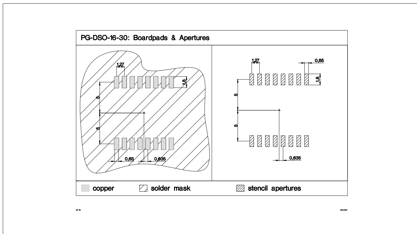
Figure 20 PG-DSO-16-30 footprint
