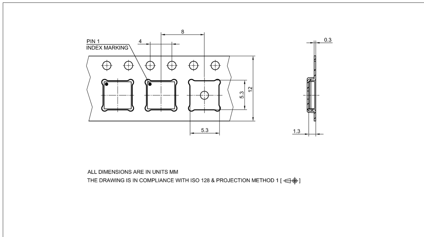
Figure 24 PG-TFLGA-13-1 packaging
