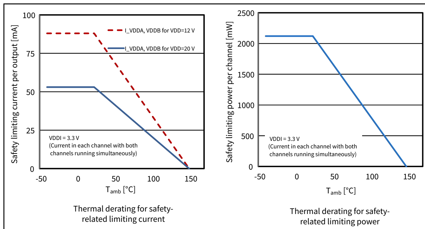
Figure 15 Thermal derating curves
