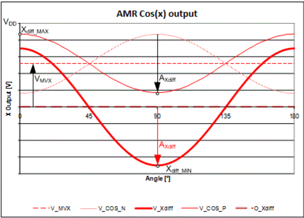
Figure 18 AMR differential output of ideal cosine
