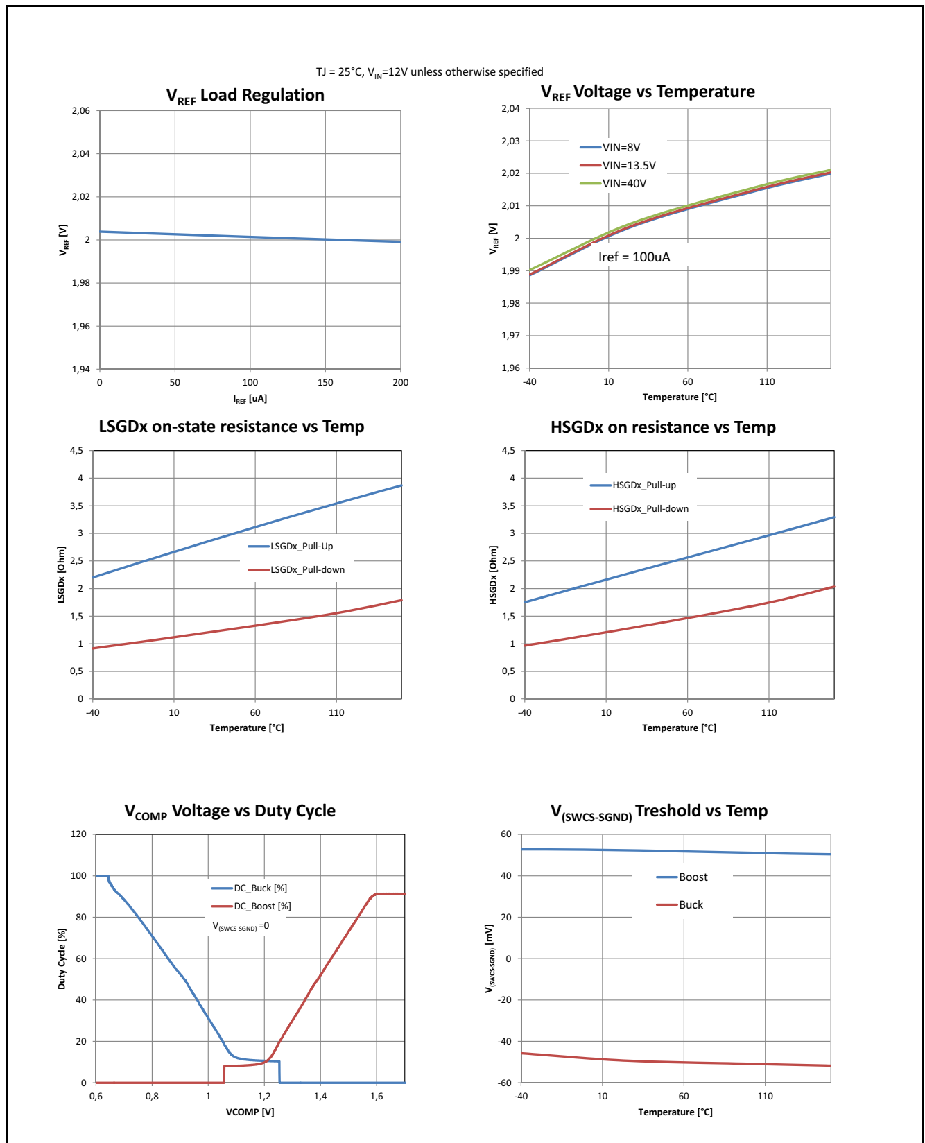
Figure 35 Characterization Diagrams 4
