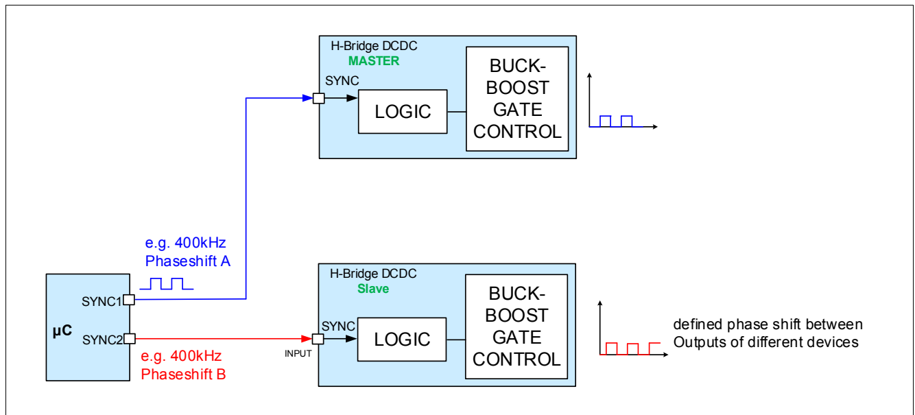
Figure 27 Synchronization Overview
