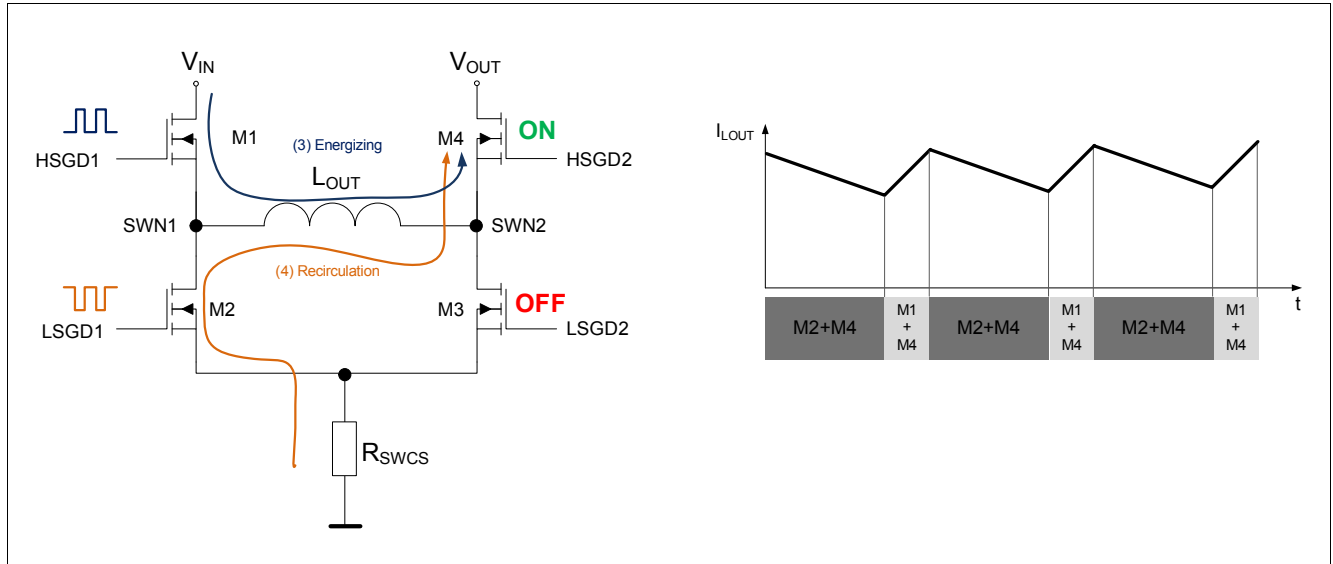
Figure 12 4 switches H-Bridge architecture in BUCK mode
