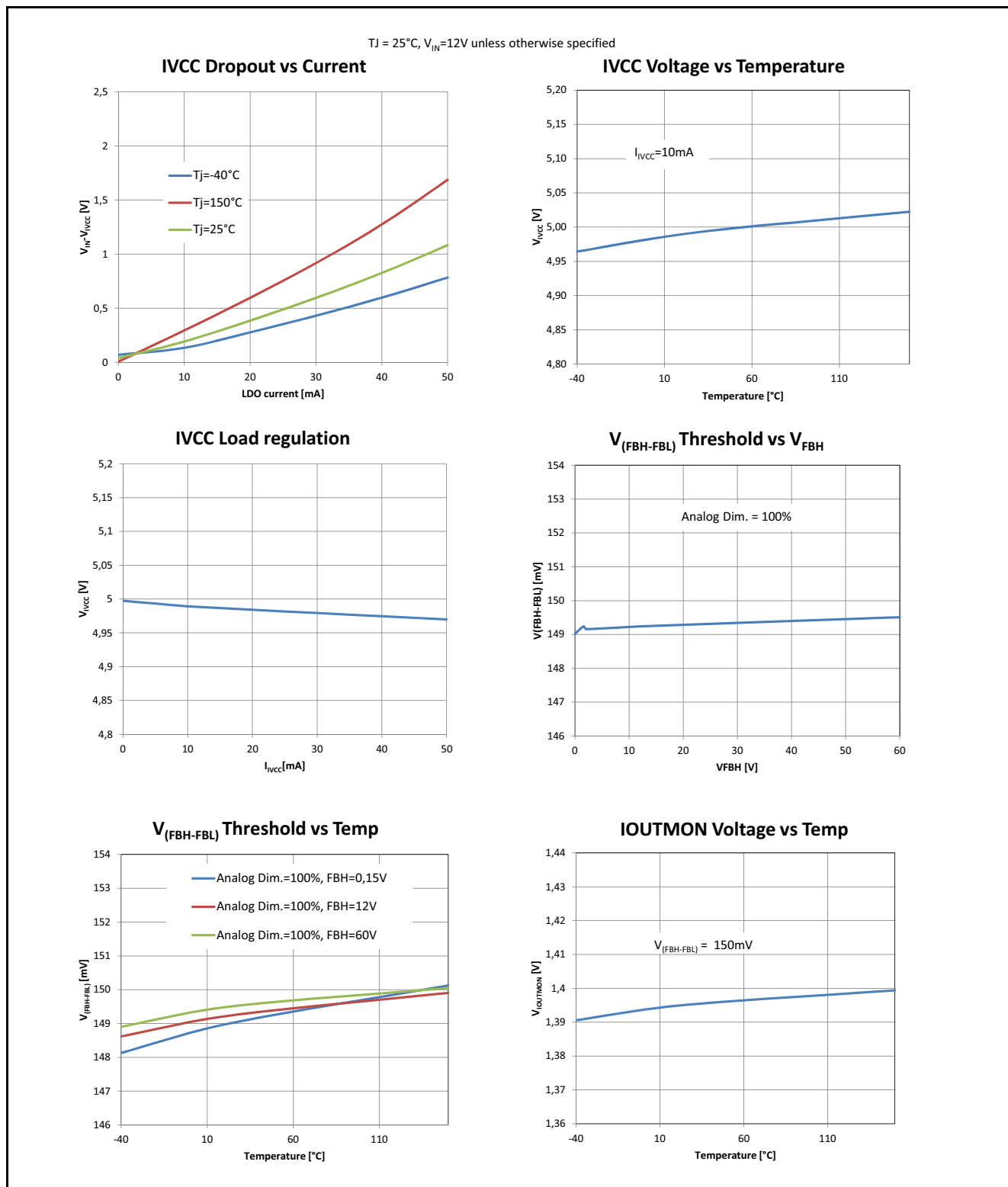
Figure 33 Characterization Diagrams 2
