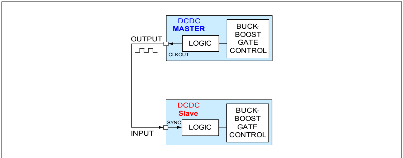
Figure 28 CLKOUT Overview
