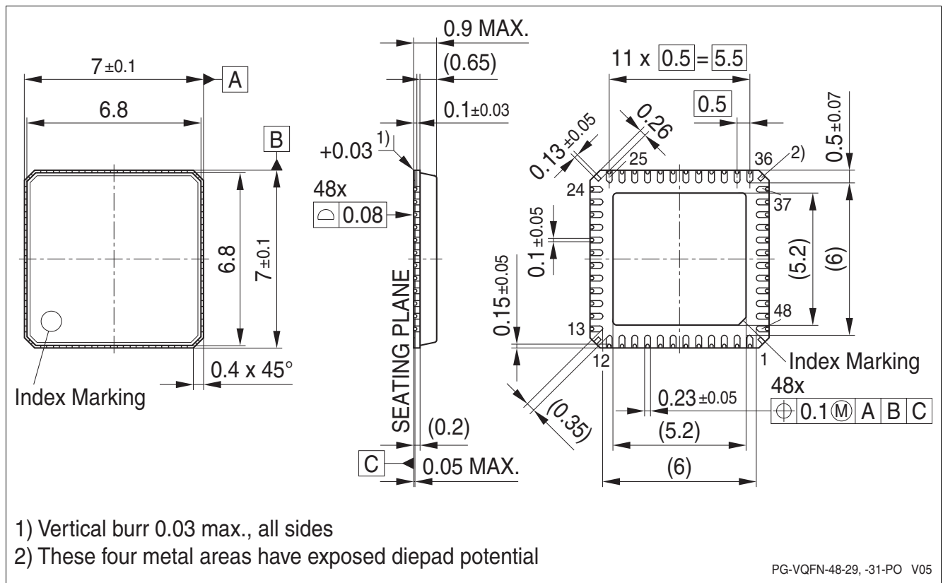
Figure 36 PG-VQFN-48-31 (with LTI)
