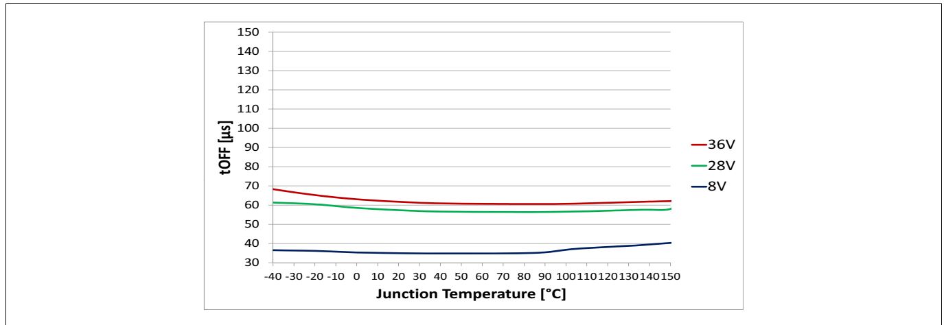
Figure 39 Turn OFF t_{\text{OFF}} = f(T_J; V_S) , R_L = 12 \Omega
