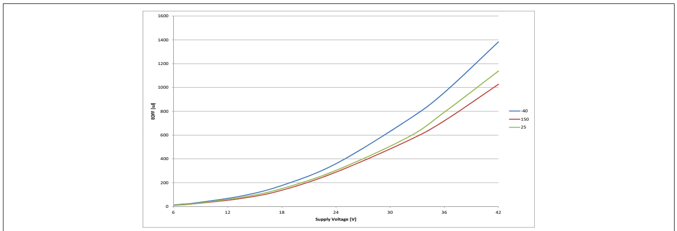
Figure 42 Switch OFF Energy E_{OFF} = f(T_J; V_S) , R_L = 12 \Omega
