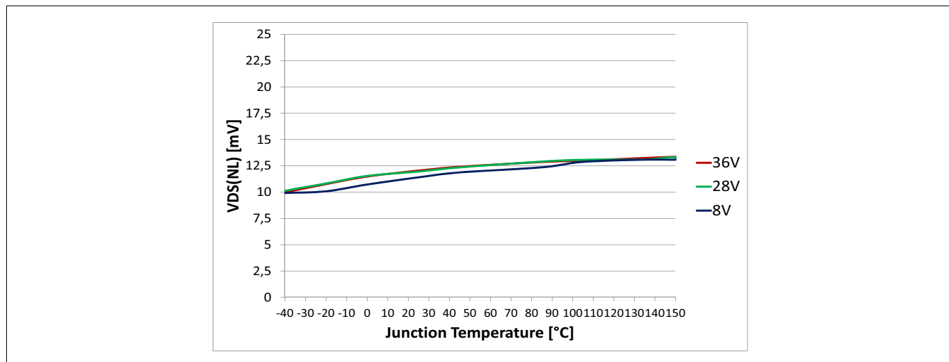
Figure 34 Output Voltage Drop Limitation at Low Load Current V_{DS(NL)} = f(T_J; V_G) ; I_L = I_{L(0)} = 50 \text{ mA}
