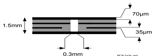
Figure 4 2s2p PCB Cross Section
