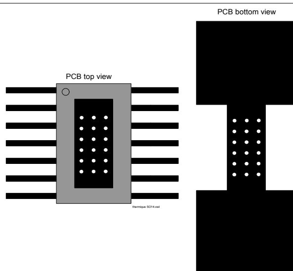
Figure 5 PC Board Top and Bottom View for Thermal Simulation with 600 mm² Cooling Area
