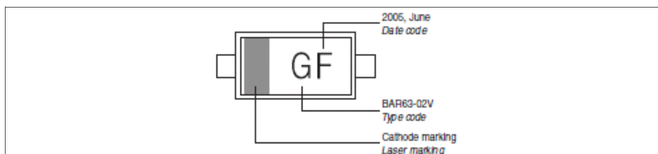
Figure 12 SC79: Marking (example)
