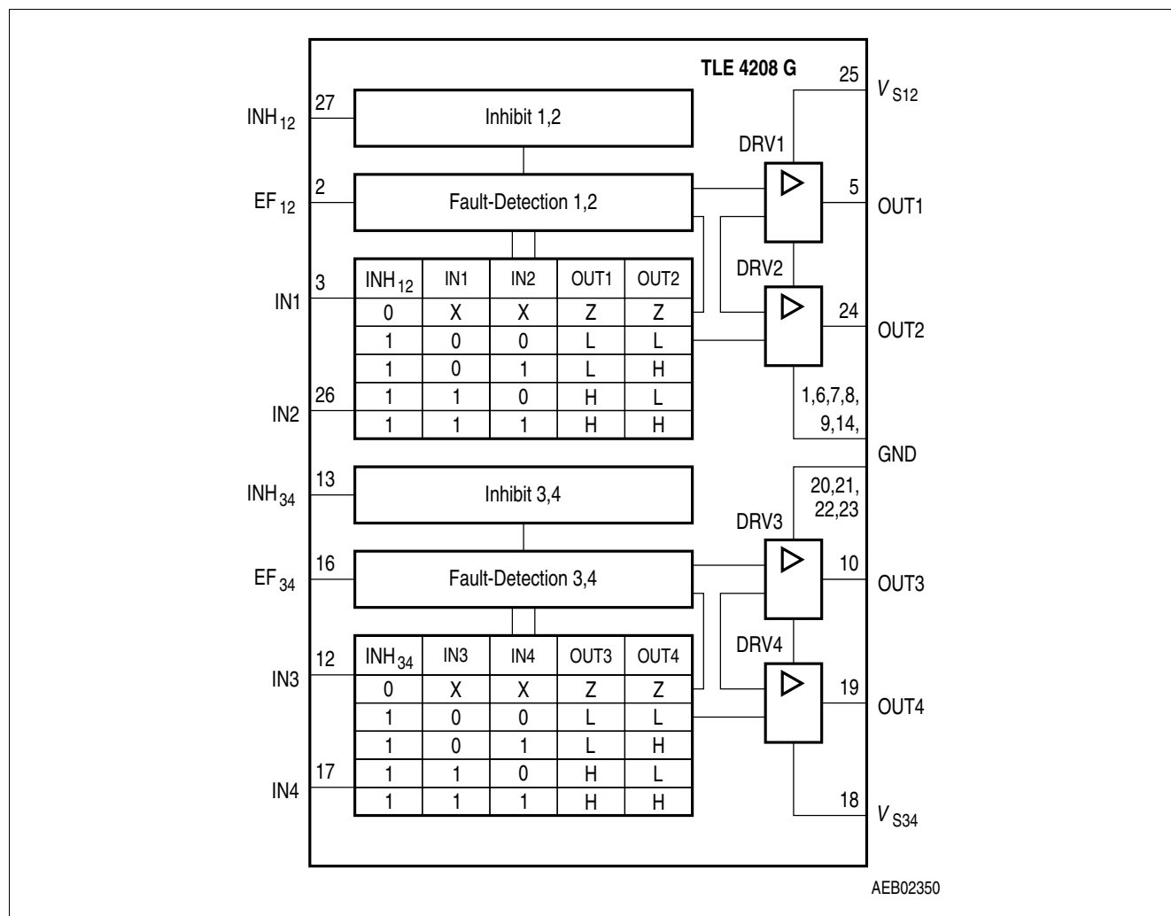
Figure 1 Block Diagram
