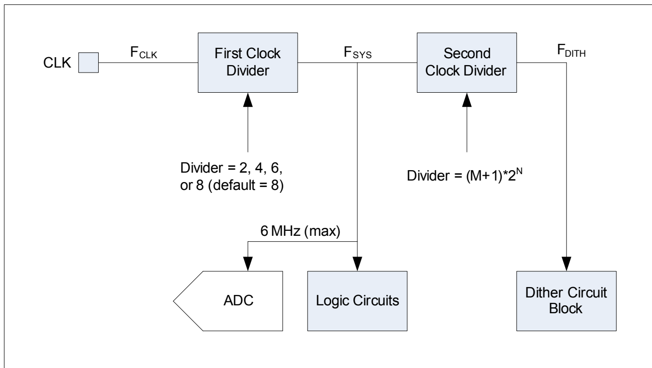
Figure 5 Clock Divider
