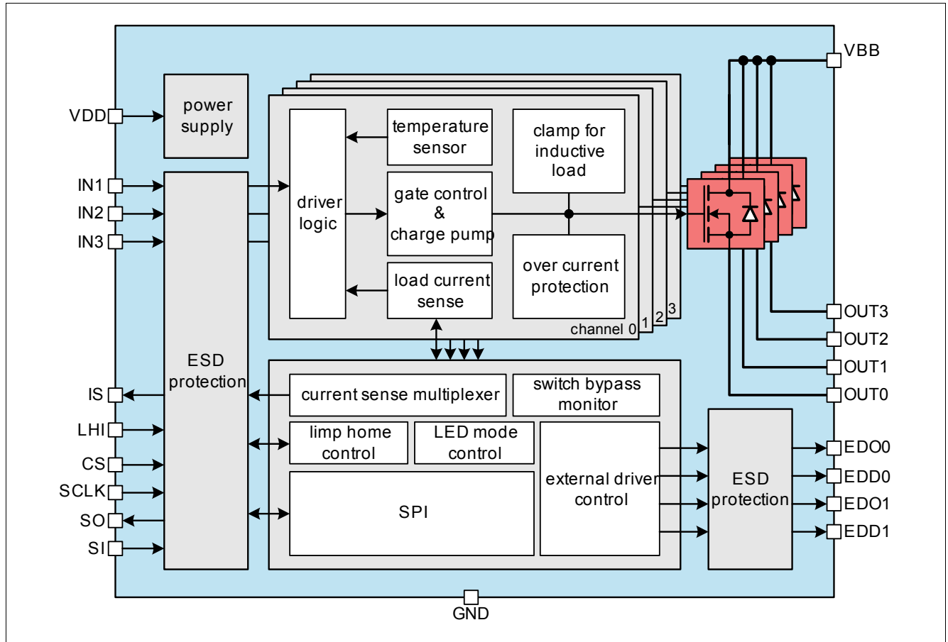
Figure 1 Block Diagram SPOC - BTS5480SF
