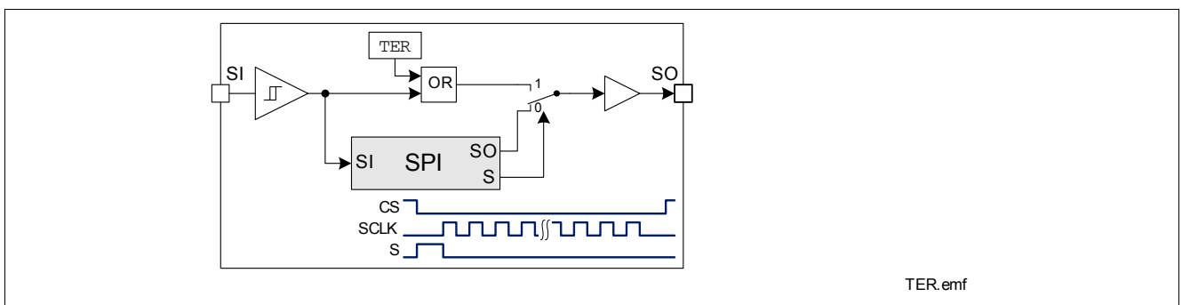
Figure 22 Combinatorial Logic for \overline{\text{TER}} Flag
