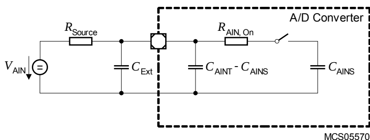
Figure 3-1 Equivalent Circuitry for Analog Inputs
