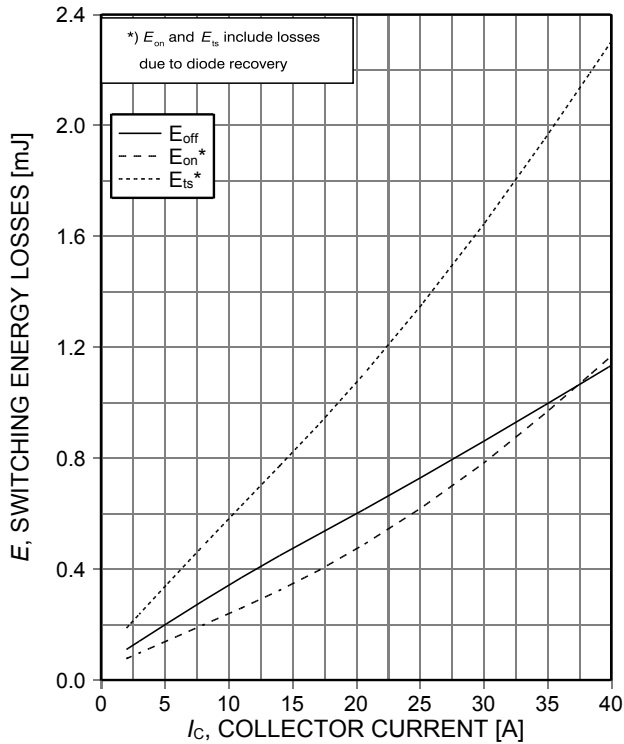
Figure 13. Typical switching energy losses as a function of collector current (inductive load, T_j=150^\circ\text{C} , V_{CE}=400\text{V} , V_{GE}=15/0\text{V} , R_G=12\Omega , Dynamic test circuit in Figure E)
