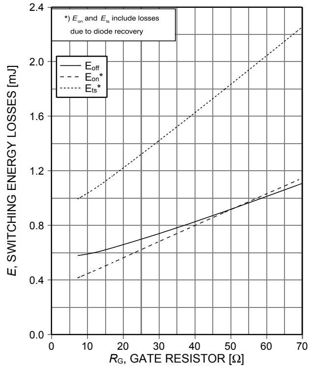
Figure 14. Typical switching energy losses as a function of gate resistor (inductive load, T_j=150^\circ\text{C} , V_{CE}=400\text{V} , V_{GE}=15/0\text{V} , I_C=20\text{A} , Dynamic test circuit in Figure E)
