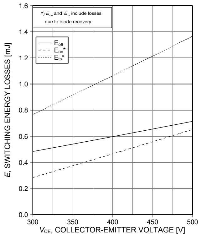
Figure 16. Typical switching energy losses as a function of collector-emitter voltage (inductive load, T_j=150^\circ\text{C} , V_{GE}=15/0\text{V} , I_C=20\text{A} , R_G=12\Omega , Dynamic test circuit in Figure E)
